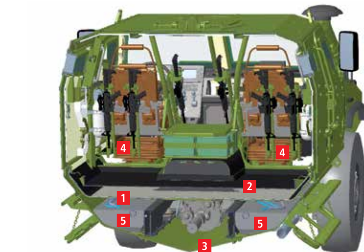
■ Vehicle section: (1) floor, (2) suspended floor, (3) V-shield, (4) anti-mine seats with side and ceiling fixtures, (5) independent fuel tanks
