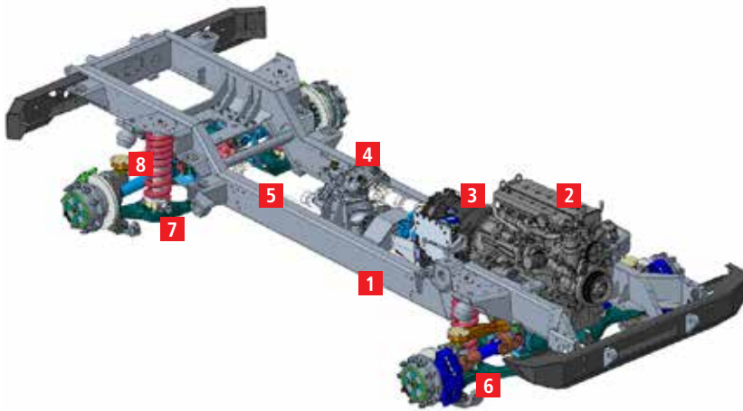
■ Diagram of chassis transmission: (1) frame, (2) motor, (3) gearbox, (4) descending gearbox, and (5) universal joint, (6) front axle, (7) rear axle, (8) coil suspension with hydraulic shock absorber
